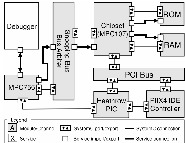
Fig. 1. Full-System PowerMac G3 simulator with debugging services.
